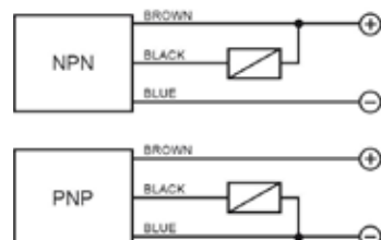
4 wires (PNP/NPN, NO/NC)
