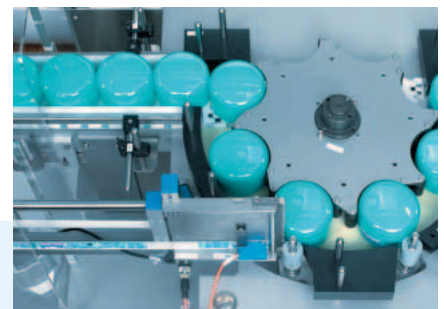
Dispensing labels in intermittently rotating star wheel – HERMA 040 M
